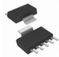
MCP1824T-1802E/DC Microchip Technology IC REG LDO 1.8V 0.3A SOT223-5
