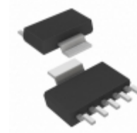
MCP1824T-2502E/DC Microchip Technology IC REG LDO 2.5V 0.3A SOT223-5
