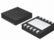
MCP4232-502E/MF Microchip Technology IC POT DGTL DUAL 5K RHEO 10DFN
