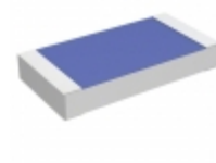
LR2010-R033FW TT Electronics/Welwyn RES SMD 0.033 OHM 1% 1W 2010
