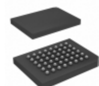
SST39LF401C-55-4C-B3KE-T Microchip Technology IC FLASH 4MBIT 55NS 48TFBGA
