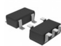
BU4909G-TR Rohm Semiconductor IC VOLT DETECTOR STD 5-SSOP
