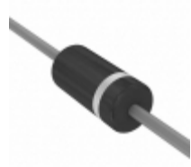
P6KE11C-E3/73 Vishay Semiconductor Diodes Division TVS DIODE 8.92VWM 16.2VC DO204AC
