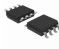
BR24S128F-WE2 LAPIS Semiconductor IC EEPROM 128KBIT 400KHZ 8SOP
