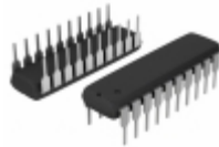
PIC16LC771-E/P Microchip Technology IC MCU 8BIT 7KB OTP 20DIP
