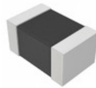
EZJ-S2VB223 Panasonic Electronic Components VARISTOR 12V 0805
