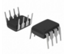
HCPL-2730-020E Broadcom Limited OPTOISO 5KV 2CH DARLINGTON 8-DIP
