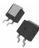
DHG30IM600PC IXYS DIODE GEN PURP 600V 30A TO263
