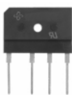
GSIB2580-E3/45 Vishay Semiconductor Diodes Division DIODE 25A 800V GSIB-5S
