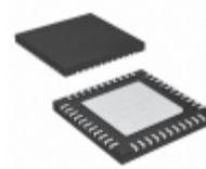
PIC24FJ64GB004T-I/ML Microchip Technology IC MCU 16BIT 64KB FLASH 44QFN
