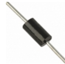
SA7V5A Fairchild/ON Semiconductor TVS DIODE 7.5VWM 12.9VC DO15
