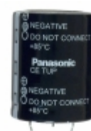
ECE-T2DP272FA Panasonic Electronic Components CAP ALUM 2700UF 20% 200V SNAP
