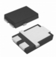
SS5P6-E3/87A Vishay Semiconductor Diodes Division DIODE SCHOTTKY 60V 5A TO277A
