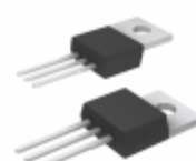
MC78M05BTG ON Semiconductor IC REG LDO 5V 0.5A TO220AB
