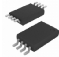
BR24C01-DW6TP Rohm Semiconductor IC EEPROM 1KBIT 400KHZ 8TSSOP
