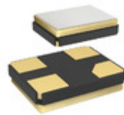
FA-20H 27.1200MA10V-C3 EPSON CRYSTAL 27.1200 MHZ 18.0PF SMD
