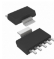
MCP1826T-3002E/DC Microchip Technology IC REG LDO 3V 1A SOT223-5
