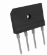
GBJ2504-G Comchip Technology BRIDGE DIODE 25A 400V GBJ
