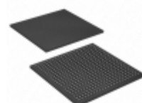
EP4CE115F23I7N Intel® FPGAs IC FPGA 280 I/O 484FBGA
