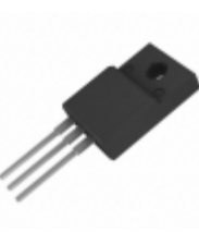
FQPF9N25CT Fairchild/ON Semiconductor MOSFET N-CH 250V 8.8A TO-220F
