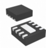
LT3060EDC-1.5#TRPBF Linear Technology IC REG LDO 1.5V 0.1A 8DFN
