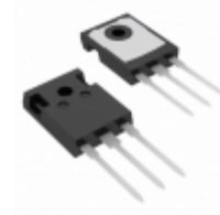
FGH40N60UFTU Fairchild/ON Semiconductor IGBT 600V 80A 290W TO247
