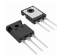
FGH40N60UFD AMI Semiconductor / ON Semiconductor IGBT 600V 80A 290W TO247
