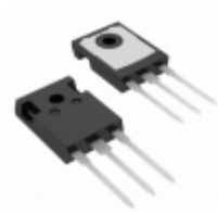
FGH40N60SMD_F085 Fairchild/ON Semiconductor IGBT 600V 80A 349W TO-247-3
