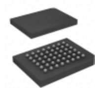
SST39VF401C-70-4I-B3KE Microchip Technology IC FLASH 4MBIT 70NS 48TFBGA
