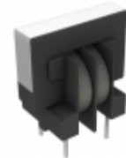
UF1717H-103YR25-01 TDK Corporation CMC 10MH 250MA 2LN TH
