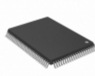
IS61NLP12836EC-200TQLI-TR ISSI, Integrated Silicon Solution Inc IC SRAM 4.5MBIT 200MHZ 100TQFP
