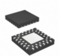
ATMEGA324PV-10MCU Microchip Technology IC MCU 8BIT 32KB FLASH 44QFN
