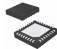
PIC16F1782-I/MV Microchip Technology IC MCU 8BIT 3.5KB FLASH 28UQFN
