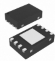
11LC020T-I/MNY Microchip Technology IC EEPROM 2KBIT 100KHZ 8TDFN
