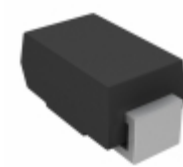
P4SMA110A-E3/61 Vishay Semiconductor Diodes Division TVS DIODE 94VWM 152VC SMA
