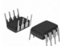
AT24C64-10PI-2.5 Microchip Technology IC EEPROM 64KBIT 400KHZ 8DIP
