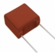
ECW-F2W225JA Panasonic Electronic Components CAP FILM 2.2UF 5% 450VDC RADIAL
