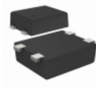
S-80124ALPF-JAJT2U SII Semiconductor Corporation IC VOLT DETECTOR 2.4V SNT-4A
