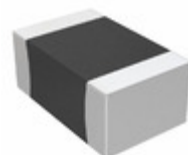
CC0805MRY5V6BB475 Yageo CAP CER 4.7UF 10V Y5V 0805
