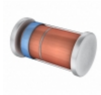
CLL4759A TR Central Semiconductor DIODE ZENER 62V 1W MELF
