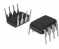
MCP3202-BI/P Microchip Technology IC ADC 12BIT 2.7V 2CH SPI 8-DIP
