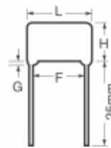
ECQ-P1H392GZ3 Panasonic Electronic Components CAP FILM 3900PF 2% 50VDC RADIAL
