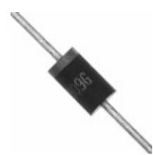
BY228GPHE3/54 Vishay Semiconductor Diodes Division DIODE GEN PURP 1.5KV 2.5A DO201
