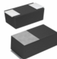
TCTAL1A336M8R Rohm Semiconductor CAP TANT 33UF 10V 20% 1206
