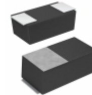
TCTAL0J107M8R Rohm Semiconductor CAP TANT 100UF 6.3V 20% 1206
