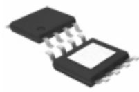
BD18GA3MEFJ-ME2 Rohm Semiconductor IC REG LDO 1.8V 0.3A 8HTSOP
