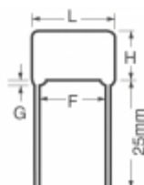
ECQ-P1H221JZ3 Panasonic Electronic Components CAP FILM 220PF 5% 50VDC RADIAL
