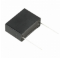
ECQ-UAAF155M Panasonic Electronic Components CAP FILM 1.5UF 20% 275VAC RADIAL
