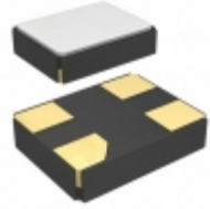
CX3225SB20000H0FLJCC AVX Corporation CRYSTAL 20.0000MHZ 12PF SMD
