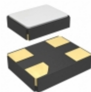
CX3225SB24000D0FPLCC Kyocera CRYSTAL 24.0000MHZ 8PF SMD
