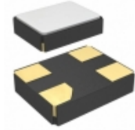
CX3225SB20000H0PSTC2 AVX Corporation CRYSTAL 20.0000MHZ 12PF SMD
