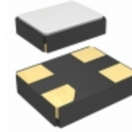
CX3225SB20000H0FLJCC Kyocera CRYSTAL 20.0000MHZ 12PF SMD
