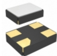
CX3225SB24000D0FFJCC AVX Corporation CRYSTAL 24.0000MHZ 8PF SMD
