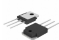
IXGQ90N33TCD1 IXYS IGBT 330V 90A 200W TO3P
