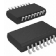
ADM3202ARWZ-REEL Analog Devices Inc. IC TXRX DUAL RS-232 3.3V 16SOIC
