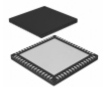
ATMEGA649P-MUR Microchip Technology IC MCU 8BIT 64KB FLASH 64QFN
