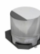
AVS158M06G24B-F Cornell Dubilier Electronics (CDE) CAP ALUM 1500UF 20% 6.3V SMD
