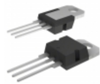
AVS12CB STMicroelectronics TRIAC INT TRIGGER 600V TO220AB
