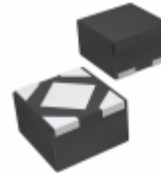
MIC5317-3.3YMT-T5 Microchip Technology IC REG LDO 3.3V 0.15A 4TDFN
